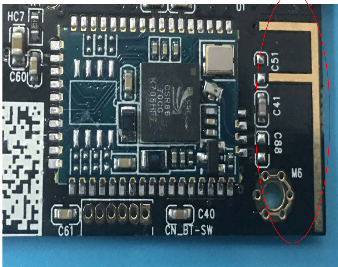
4. BT antenna view
