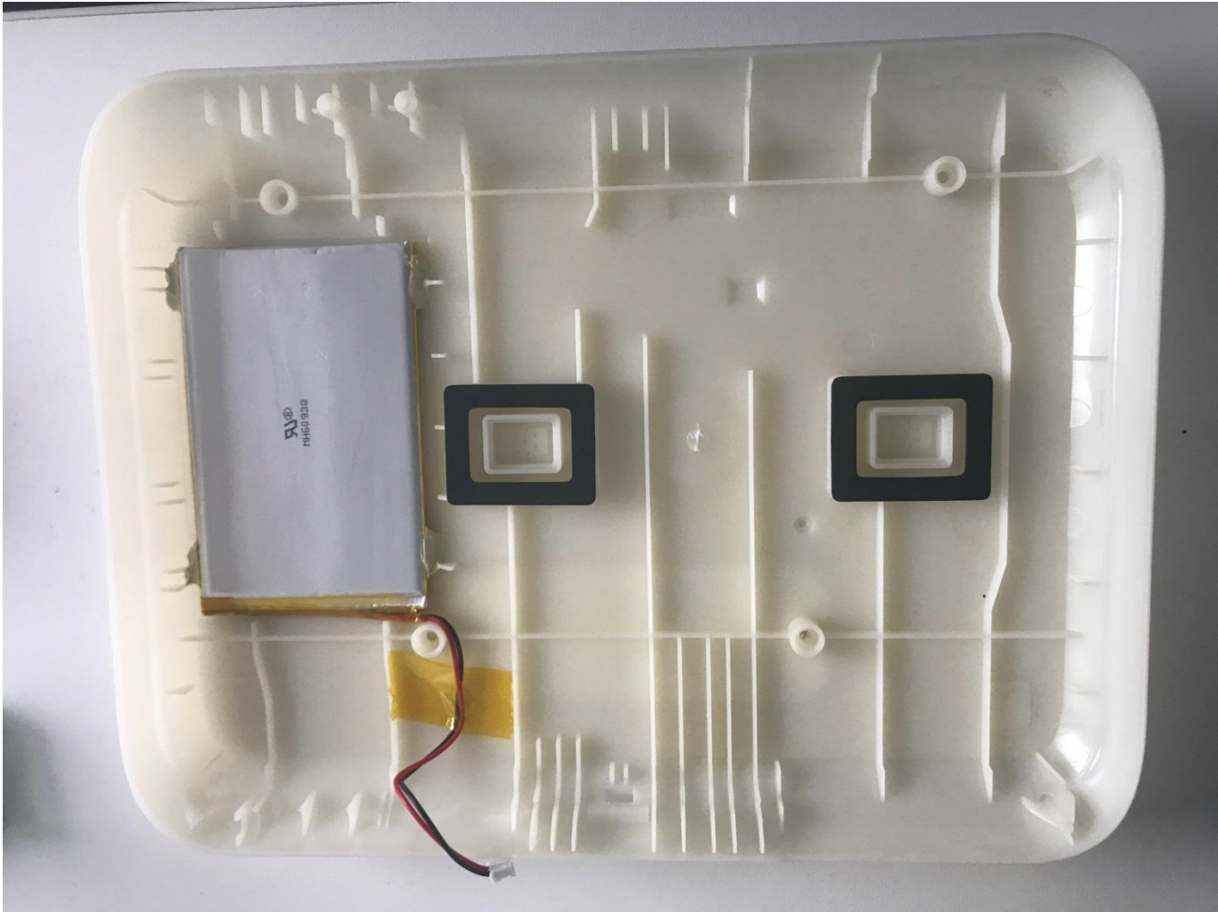
Bottom Cover
