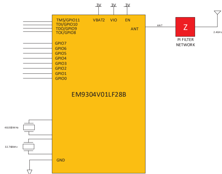
Figure 1 - 20028186 Block Diagram
