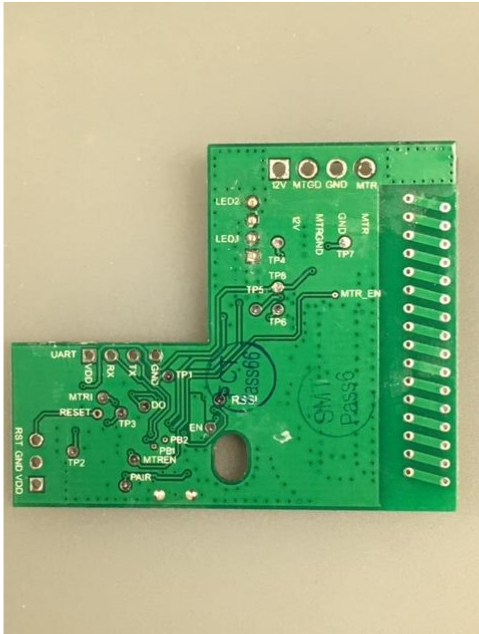
Figure 2 - WF-09 Receiver board bottom side
