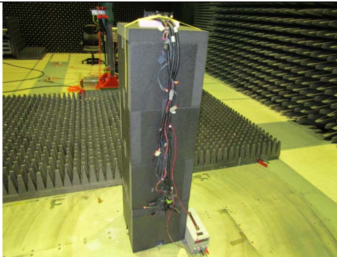
Radiated Emissions 1000-25000 MHz
