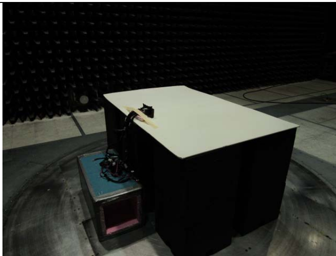
Radiated Emissions 30-1000 MHz
