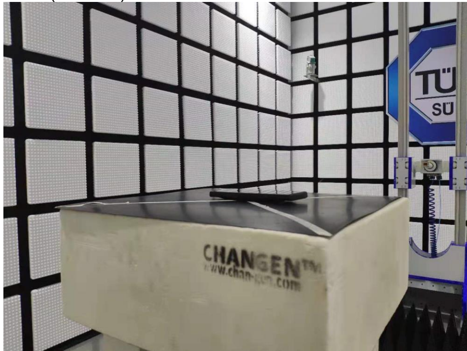
Radio Emission (18-40GHz)
