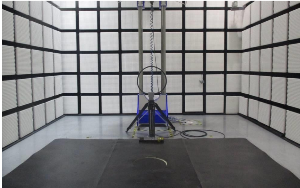
Radio Emission (9KHz-30MHz)
