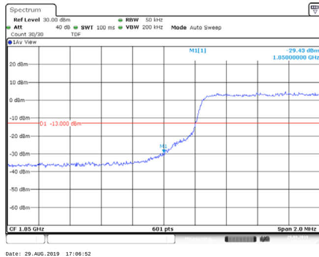
Band25_5MHz_QPSK_26665_1RB#24
