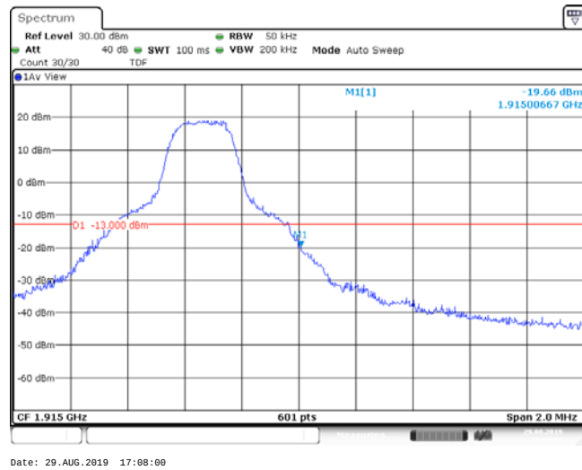
Band25_5MHz_QPSK_26665_25RB#0
