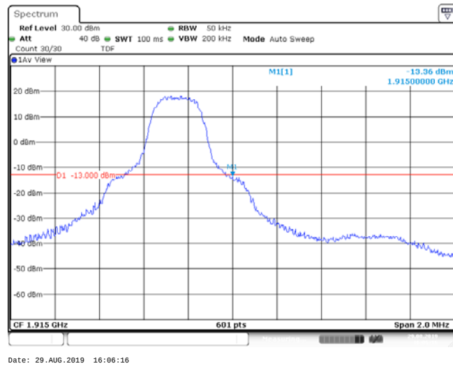
Band25_1.4MHz_16QAM_26683_6RB#0
