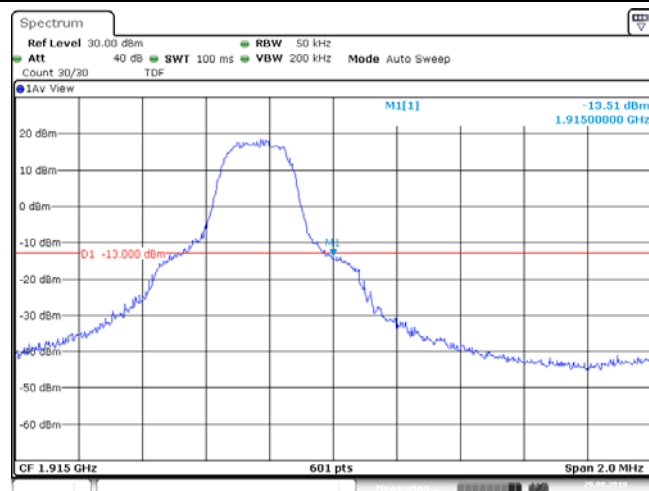
Band25_3MHz_QPSK_26675_1RB#14
