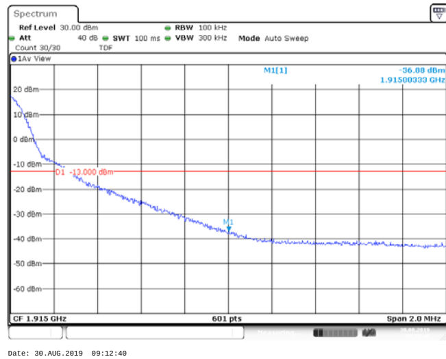
Band25_20MHz_QPSK_26590_100RB#0
