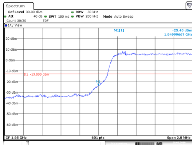
Band25_3MHz_QPSK_26055_15RB#0
