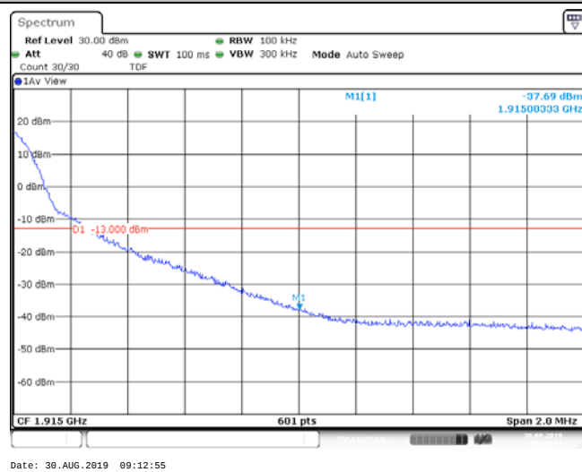
Band25_20MHz_16QAM_26590_100RB#0
