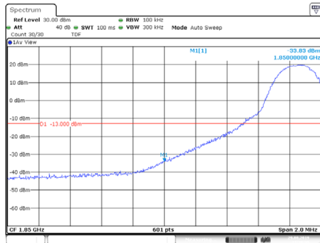
Band2_15MHz_16QAM_18675_1RB#0
