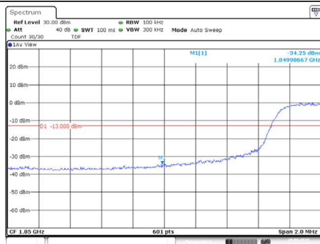
Band2_15MHz_16QAM_18675_75RB#0
