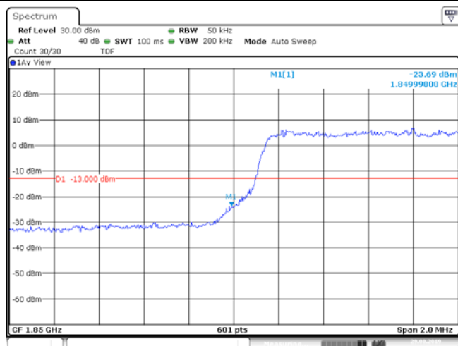
Band2_3MHz_16QAM_18615_15RB#0
