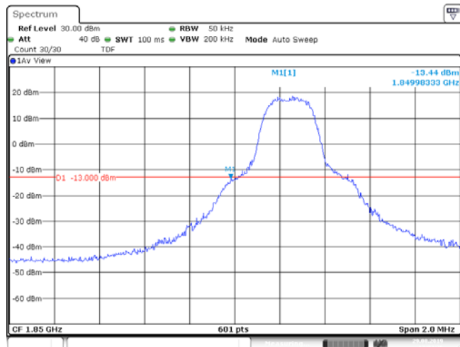
Band2_3MHz_16QAM_18615_1RB#0
