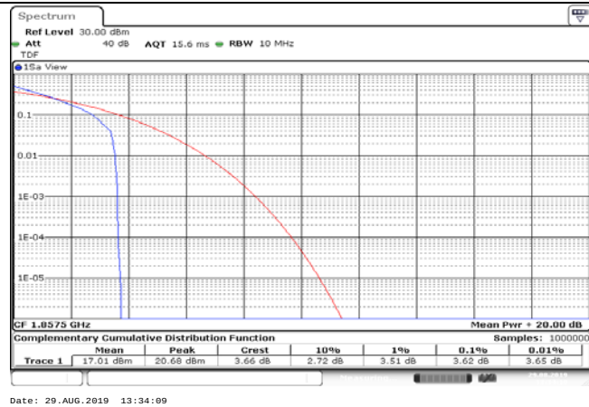
Band2_15MHz_QPSK_18675_75RB#0
