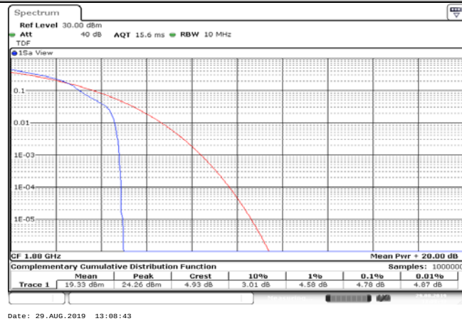
Band2_10MHz_16QAM_18900_50RB#0
