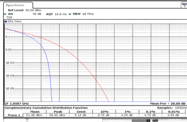
Band2_1.4MHz_QPSK_18607_6RB#0
