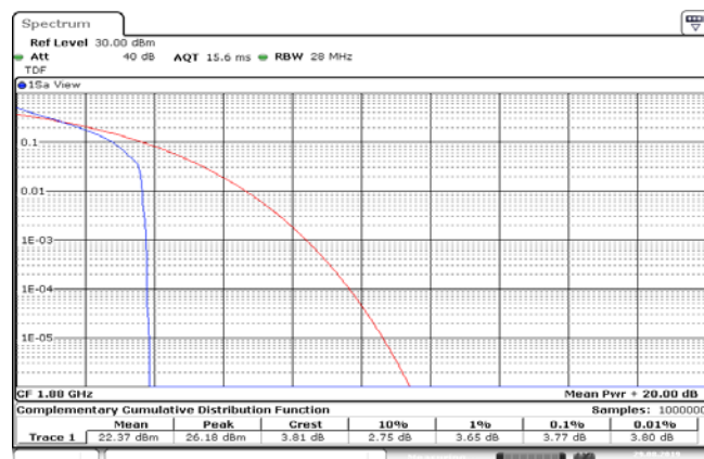
Band2_1.4MHz_QPSK_18900_1RB#0
