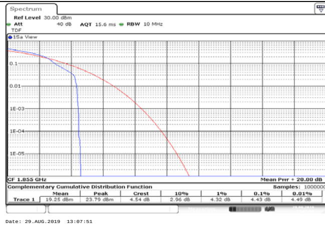
Band2_10MHz_16QAM_18650_50RB#0
