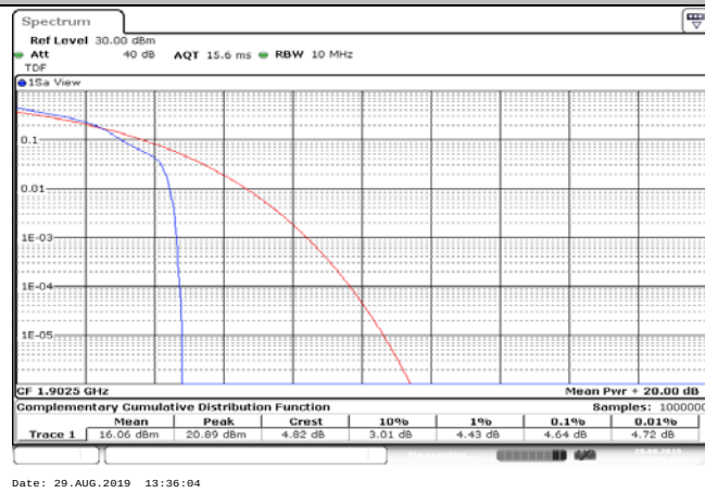
Band2_15MHz_16QAM_19125_75RB#0
