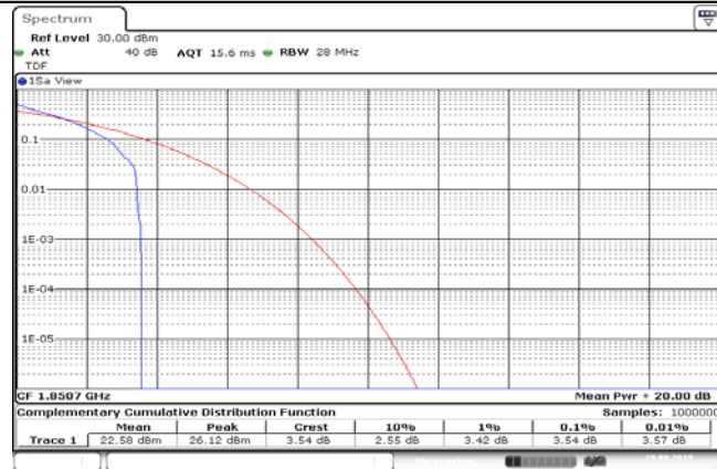
Band2_1.4MHz_QPSK_18607_1RB#0
