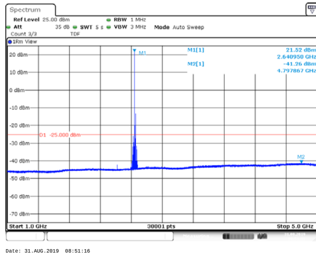
Band41_15MHz_16QAM_41165_1RB#0
