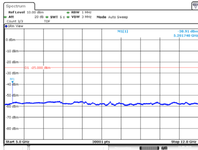
Band41_15MHz_16QAM_41165_1RB#0
