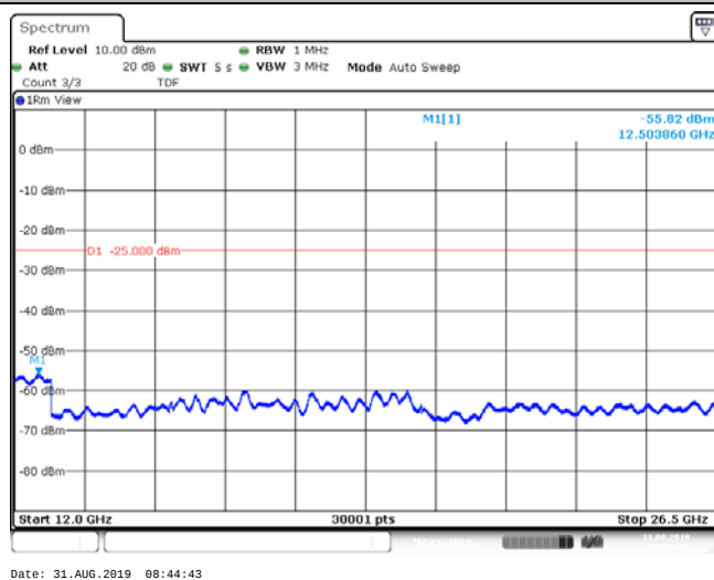
Band41_15MHz_16QAM_40740_1RB#0
