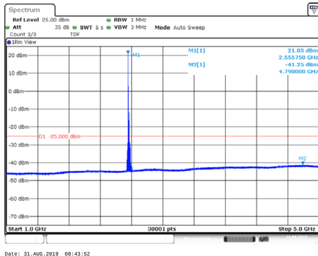
Band41_15MHz_16QAM_40315_1RB#0
