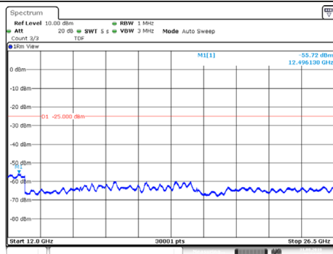
Band41_15MHz_16QAM_41165_1RB#0
