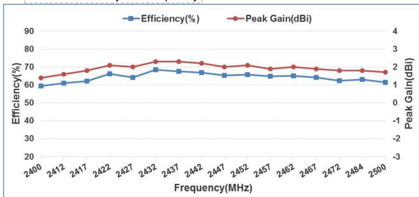
7-3. 3D Efficiency vs. Frequency
