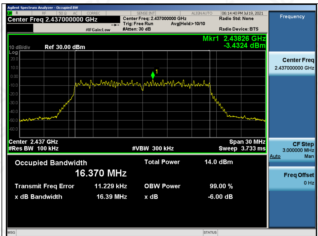
Test_Graph_802.11g_ANT1_2437_6Mbps_DTSSBW
