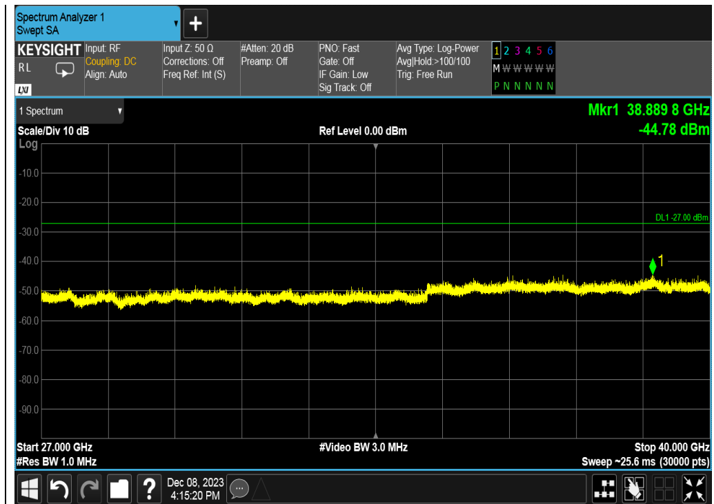
Test_Graph_802.11n40_ANT1_5270_MCS0_Frequency Band 5
