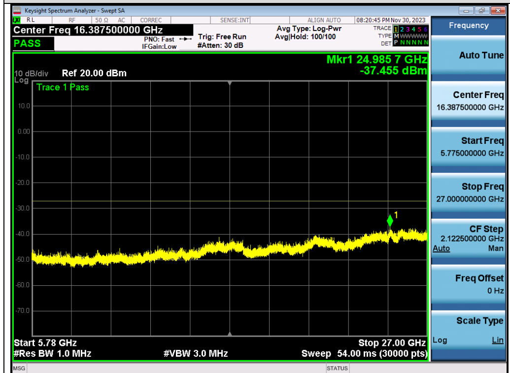
Test_Graph_802.11a_ANT1_5500_6Mbps_Frequency Band 4
