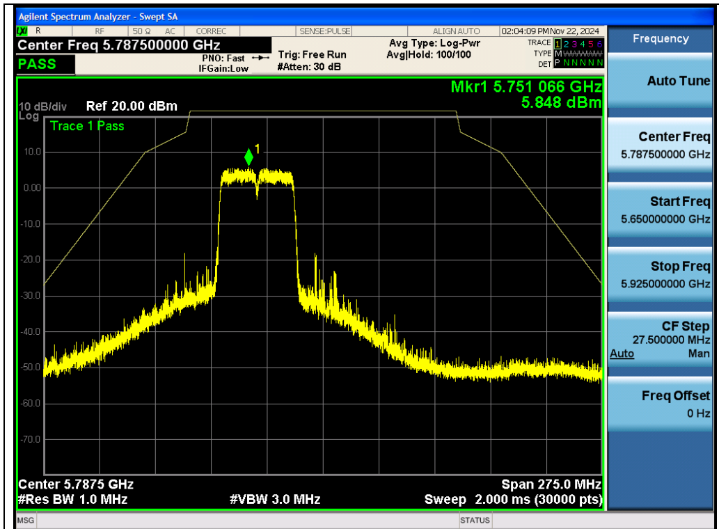
Test_Graph_802.11n40_ANT1_5755_MCS0_Frequency Band3
