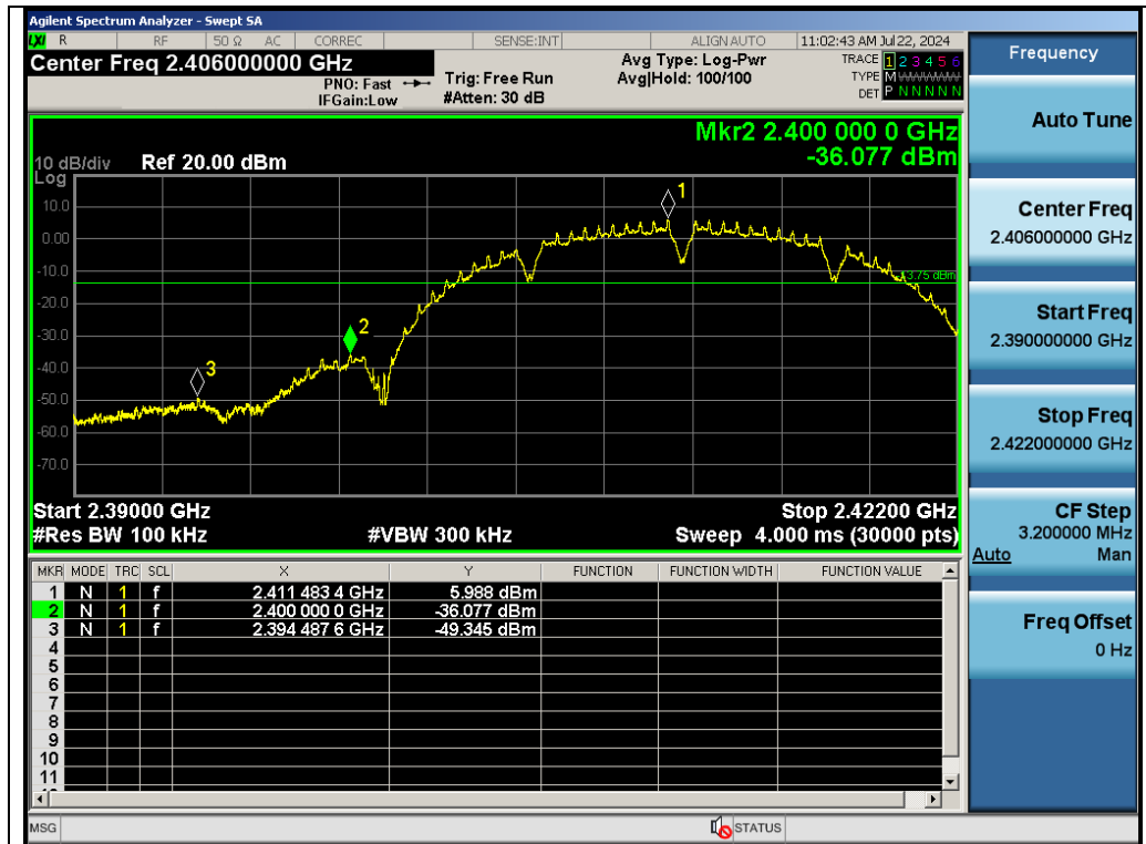
Test_Graph_802.11b_ANTA_2412_1Mbps_Lower Band Edge Emissions
