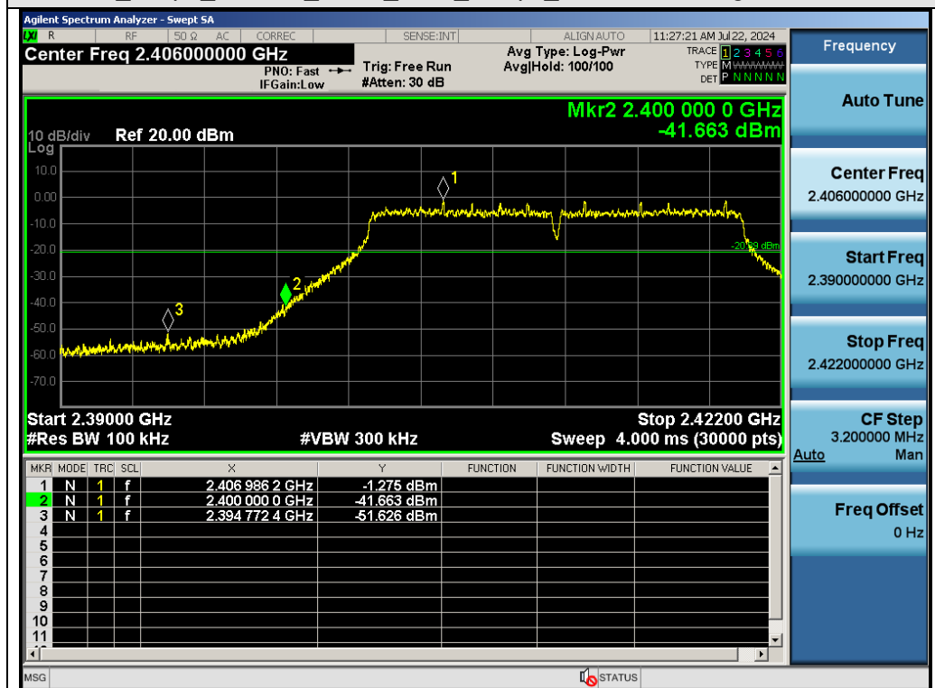
Test_Graph_802.11g_ANTA_2412_6Mbps_Lower Band Edge Emissions
