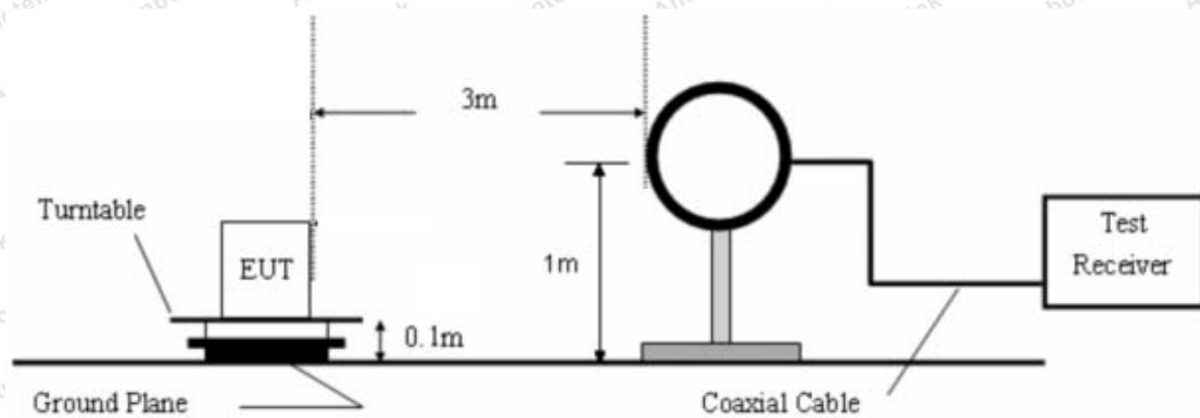
Figure 1. Below 30MHz
