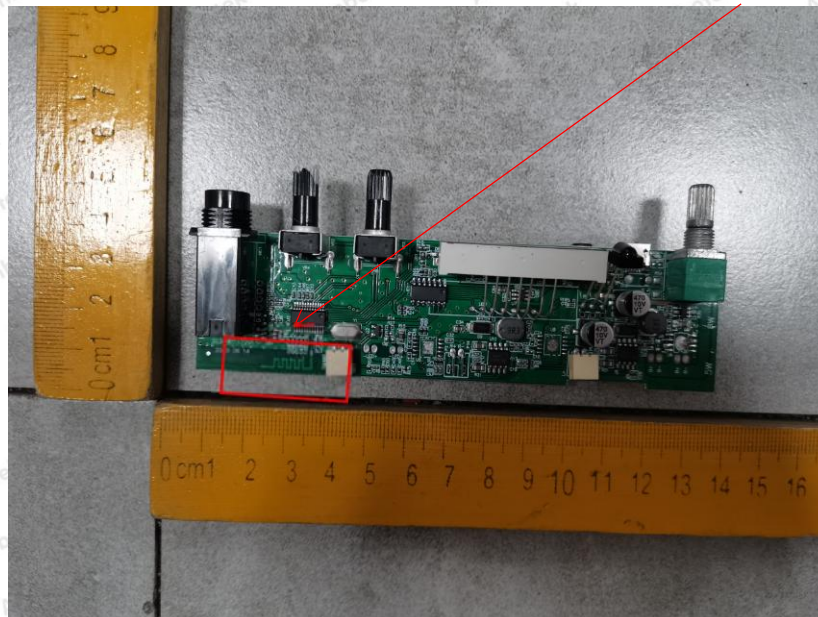
BT Antenna
