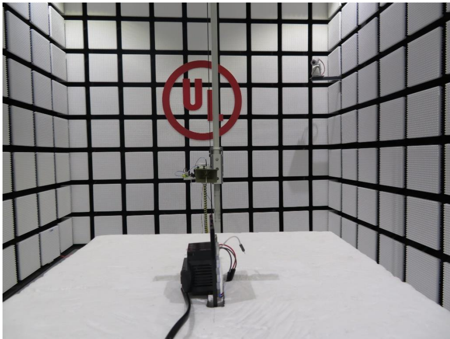
RADIATED RF MEASUREMENT POSITION (Y axis)
