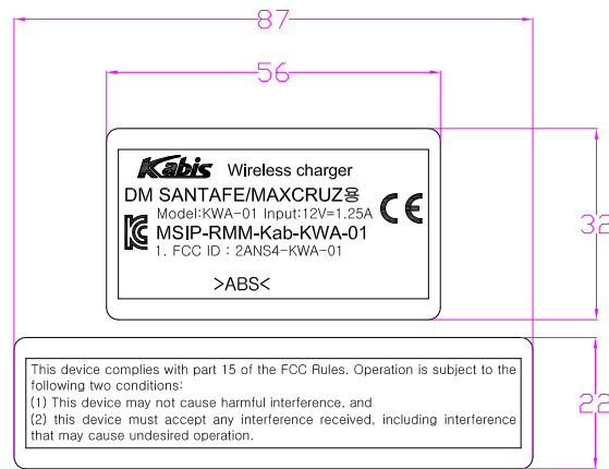
[ Label Drawing ]
