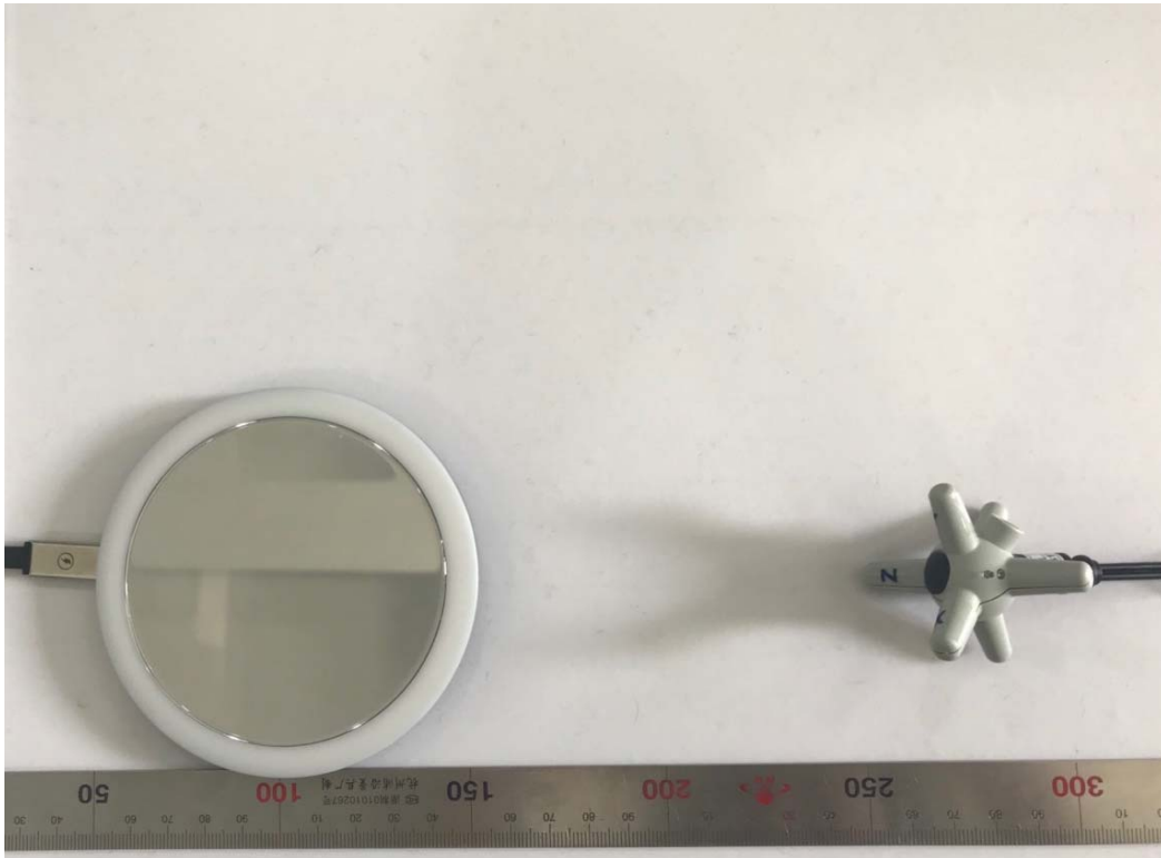
H-field Test Setup Photo
