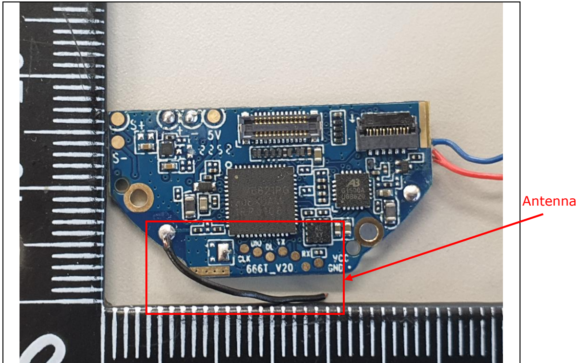
Main Board Front
