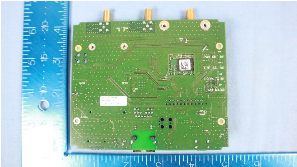
Internal Main PCB Bottom
