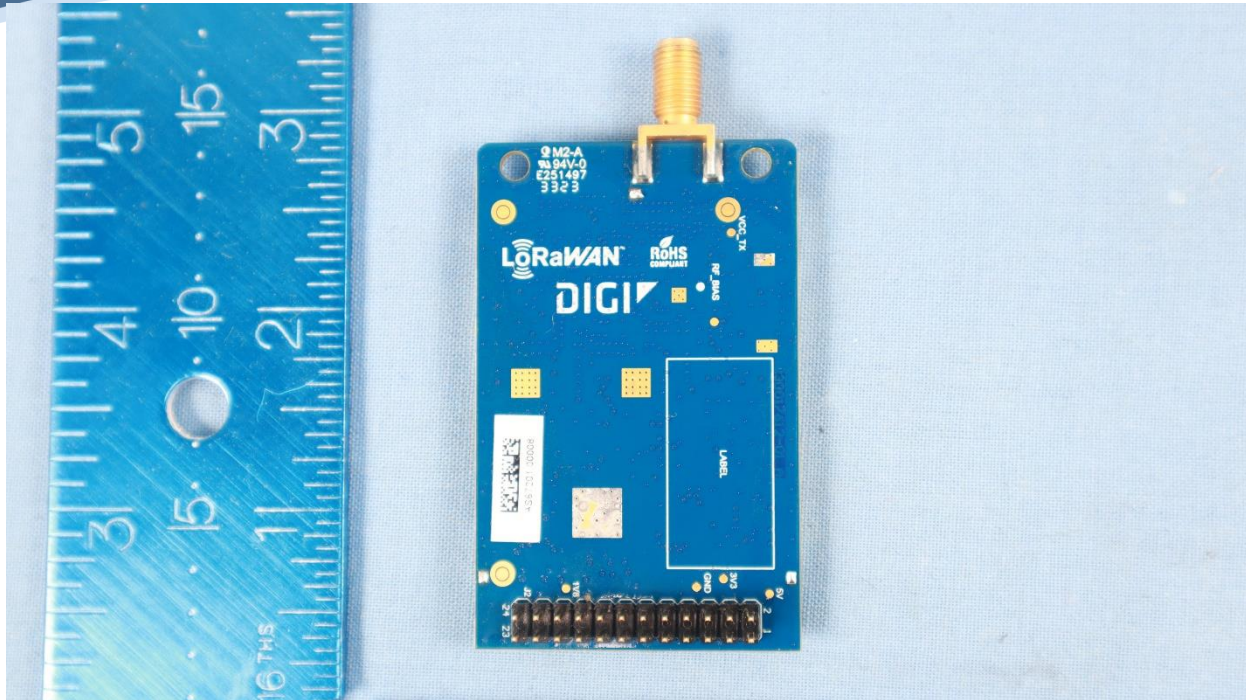
Internal Digi Radio Bottom
