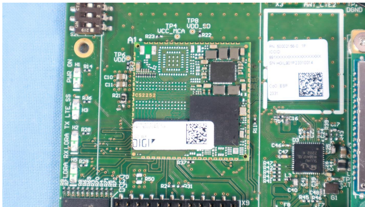
Internal Close Up Under Digi Radio
