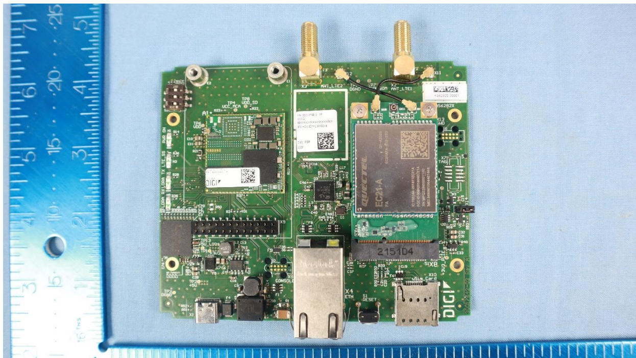
Internal Digi Radio Removed
