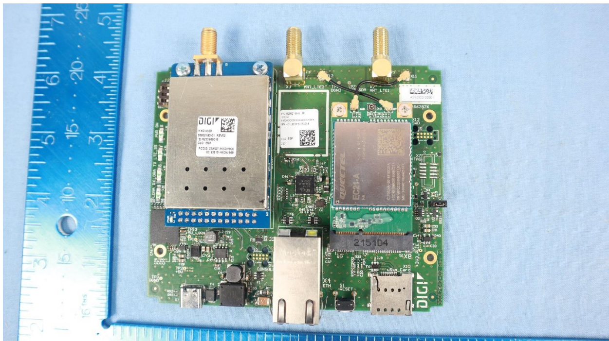
Internal Main PCB Top
