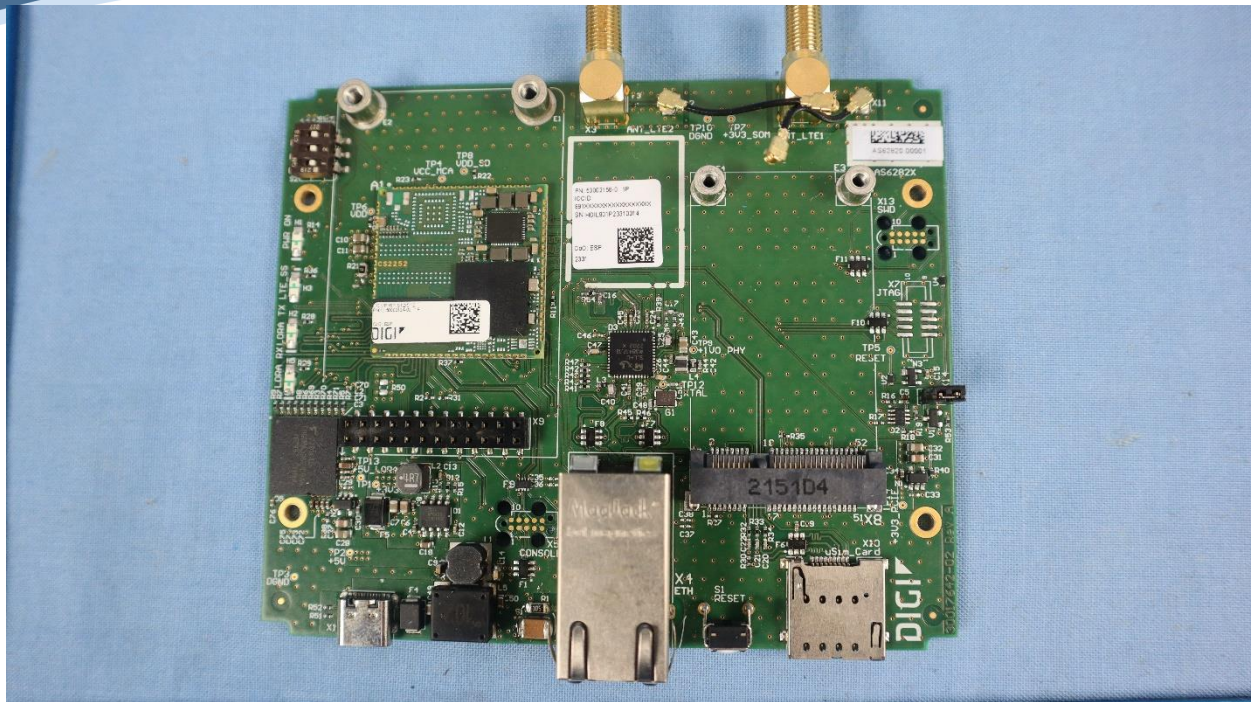
Internal Main PCB Macro
