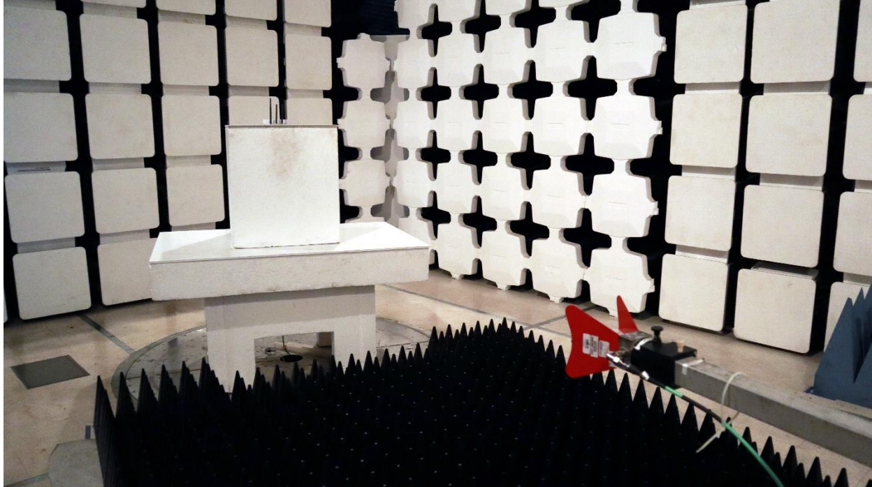
Co Location Spurious Emissions 1-18GHz
