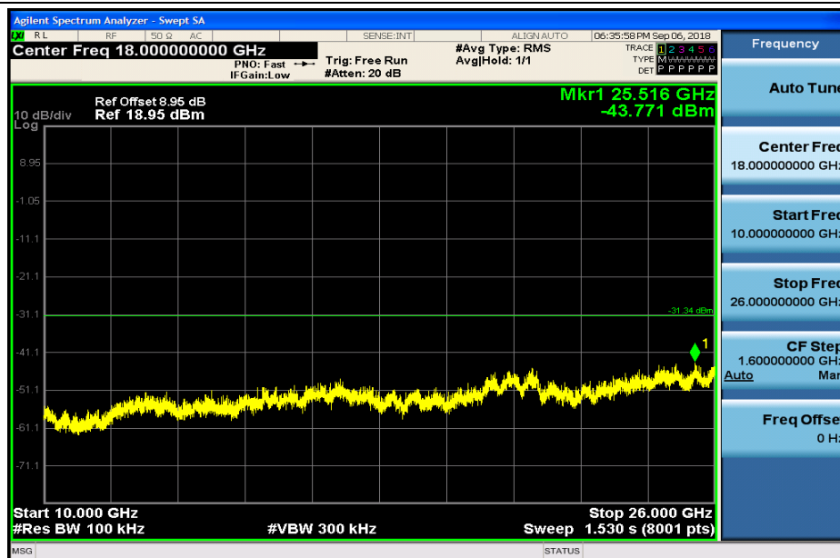
RF Conducted Spurious Emissions_11N40SISO_2437
