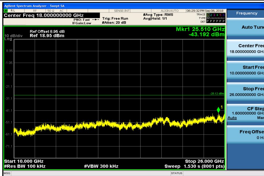
RF Conducted Spurious Emissions_11N40SISO_2422
