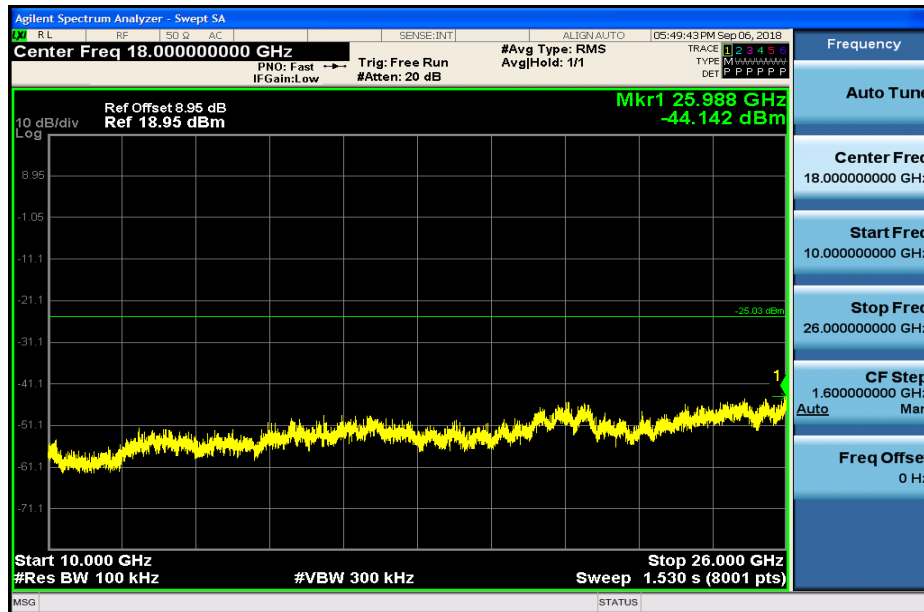
RF Conducted Spurious Emissions_11B_2462
