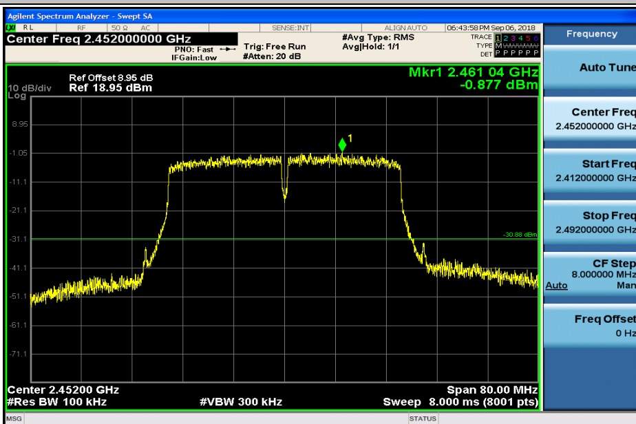
RF Conducted Spurious Emissions_11N40SISO_2452
