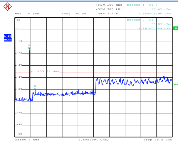
Test plot of Conducted Spurious Emission – Chain 1
