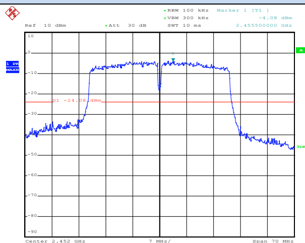
802.11n-HT40-Middle channel Reference
