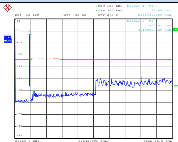
802.11n-HT40-Middle channel
