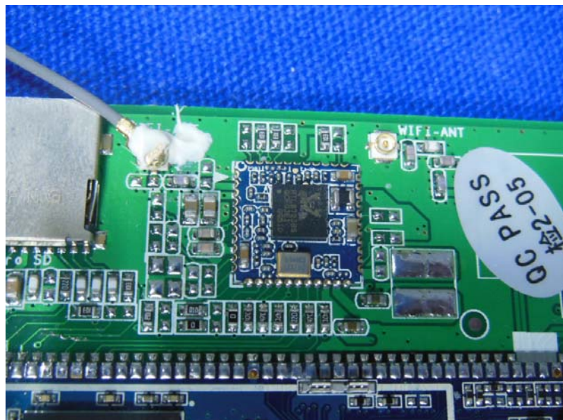
EUT –Wi-fi chip View
