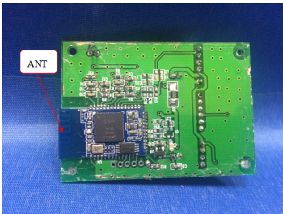
MAIN BOARD3 TOP VIEW 4
