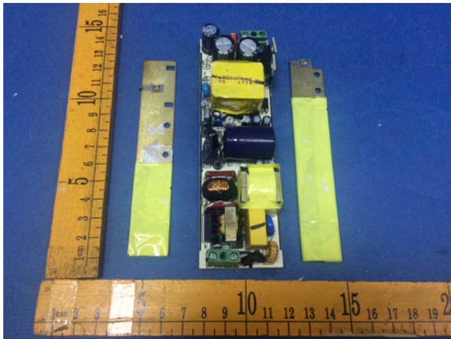
EUT UNCOVER VIEW 8
