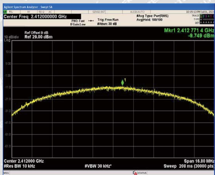
802.11b_Low Channel
