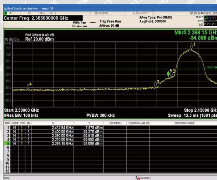
802.11b_Low Channel
