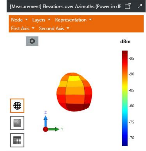
LTE B3 TIS
