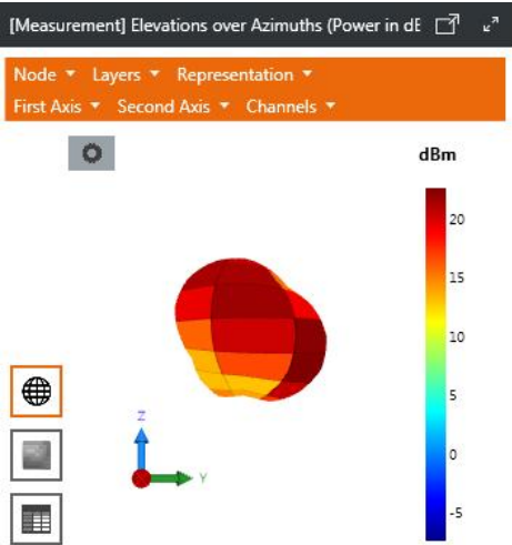
LTE B8TRP
