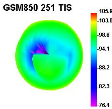
GSM850 251 TIS
