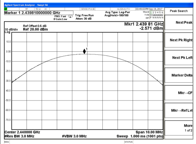
Channel 19 / 2440 MHz
