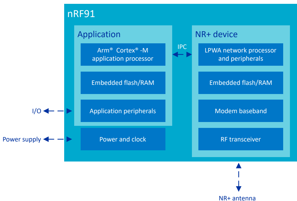
Figure 114: nRF9161 NR+ device functional overview
