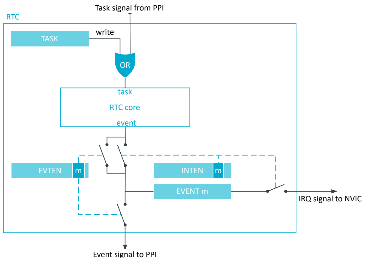
Figure 55: Tasks, events, and interrupts in the RTC
