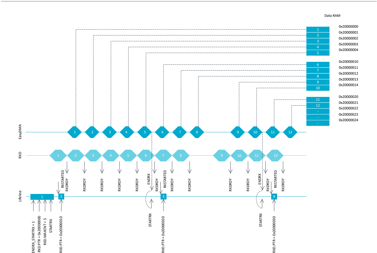
Figure 107: UARTE reception
