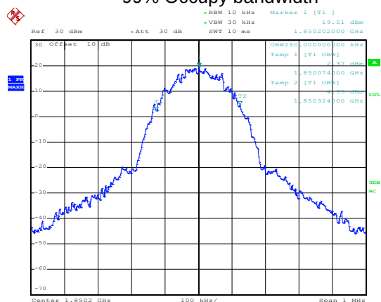
99% Occupy bandwidth
