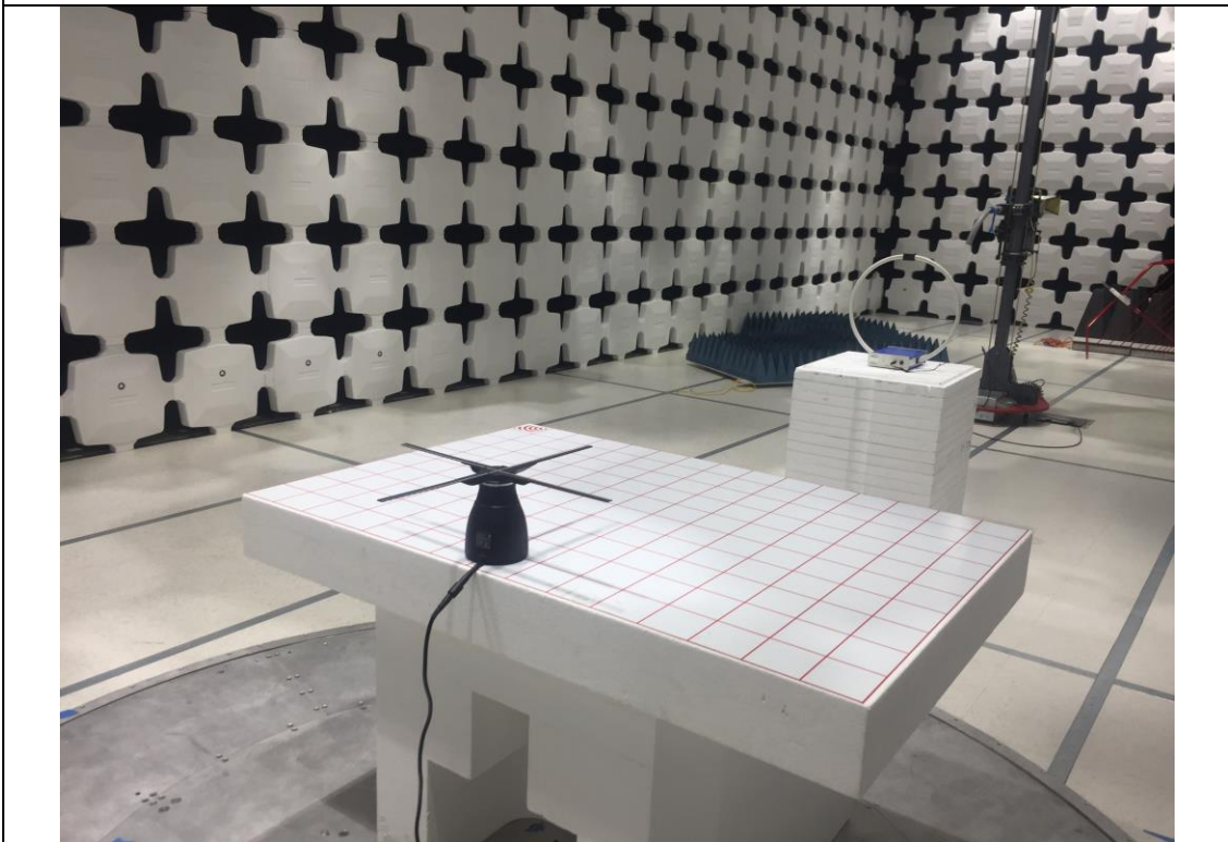
Radiated Emissions Below 30MHz setup – Rear
