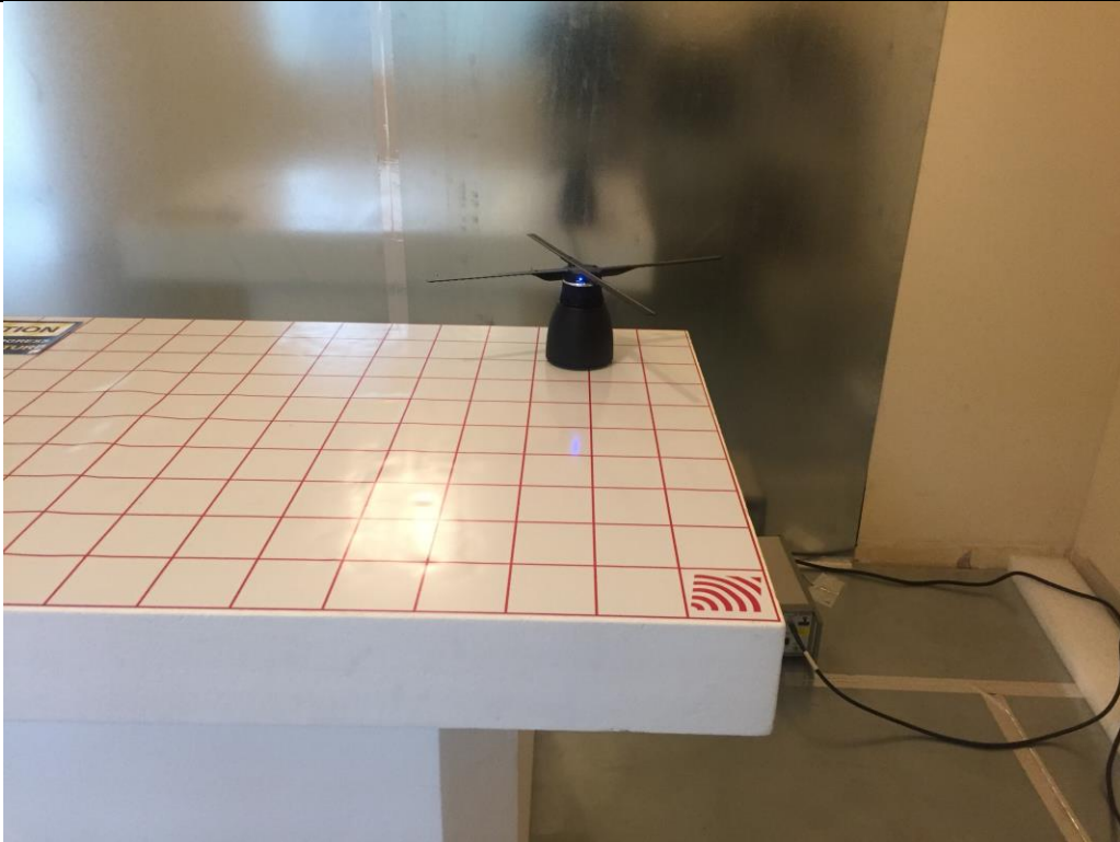
AC Line Conducted Emission setup – Front
