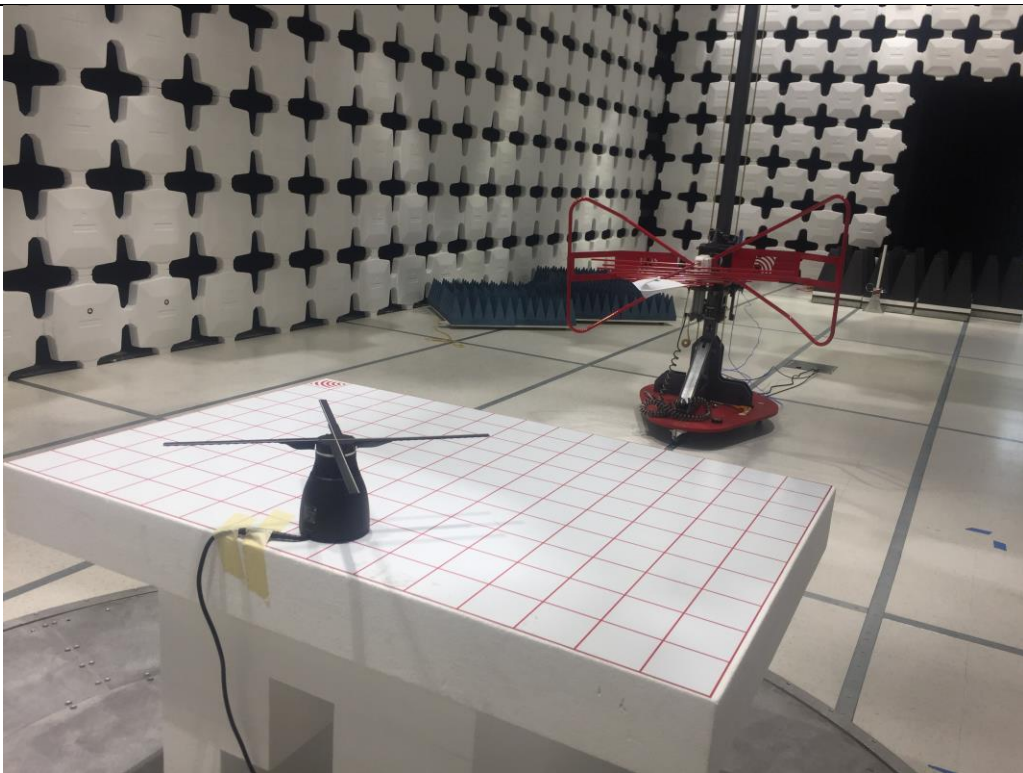
Radiated Emissions Below 1GHz setup – Rear
