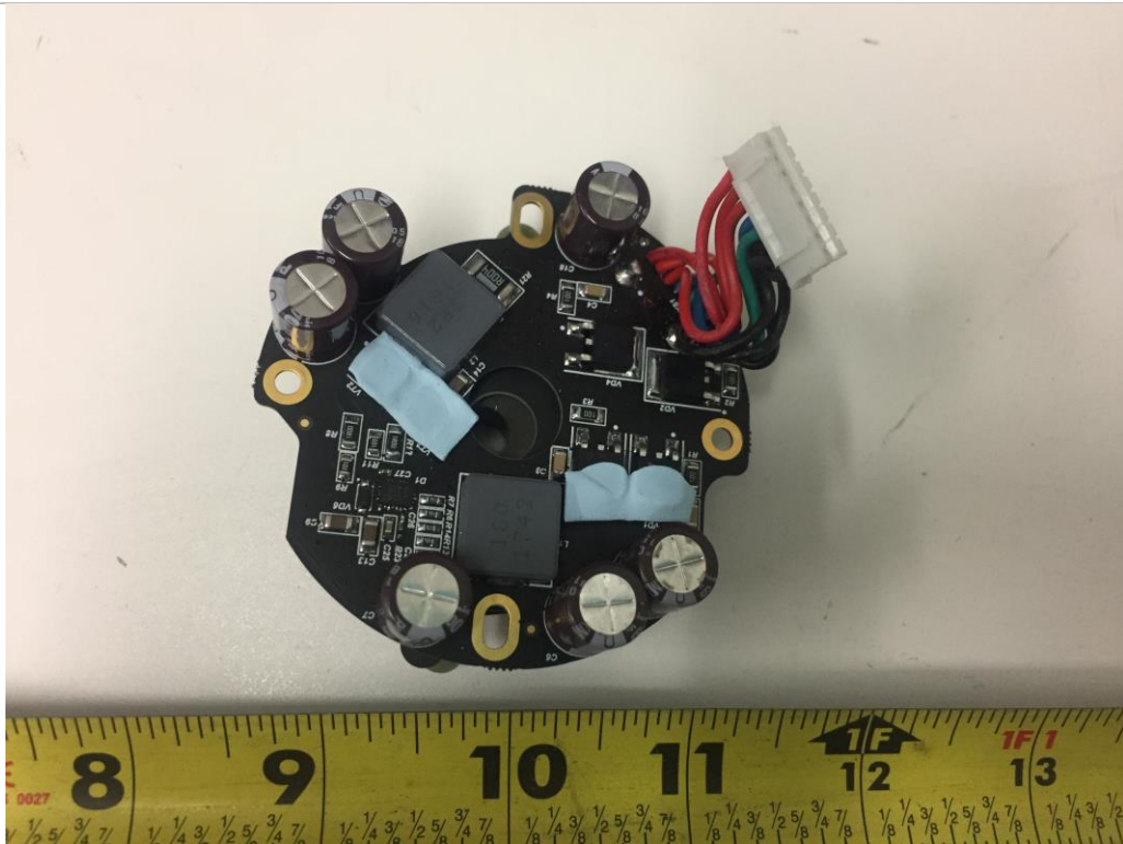
EUT PCB3 – Top View
