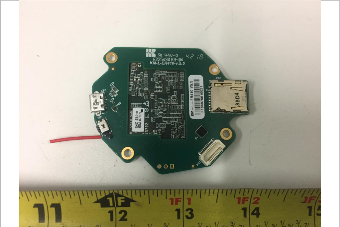
EUT PCB1 – Top View
