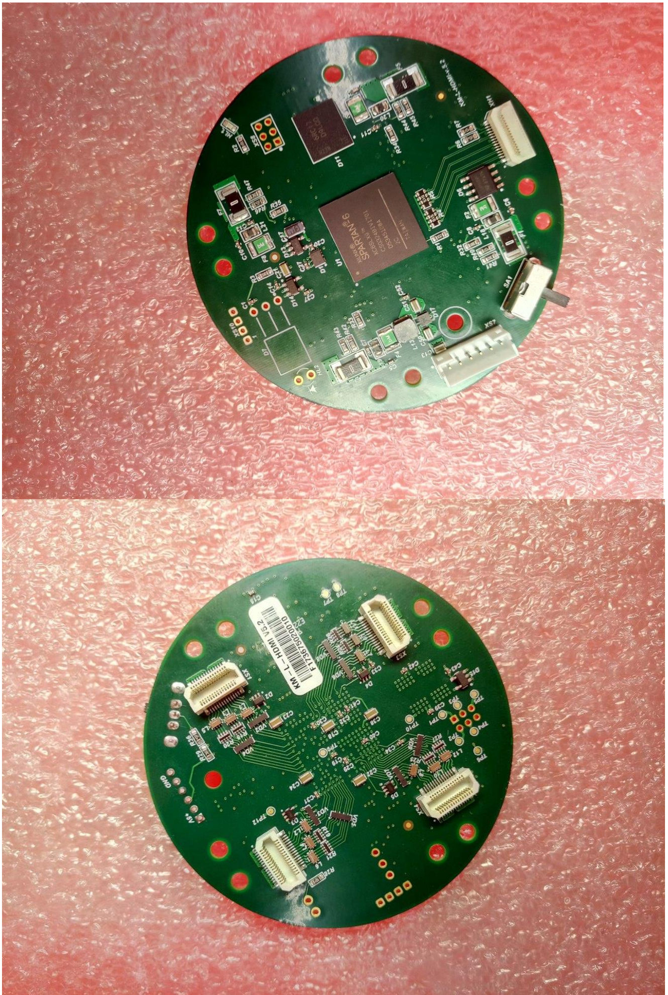
Fig 2. KM-L-HDMI
