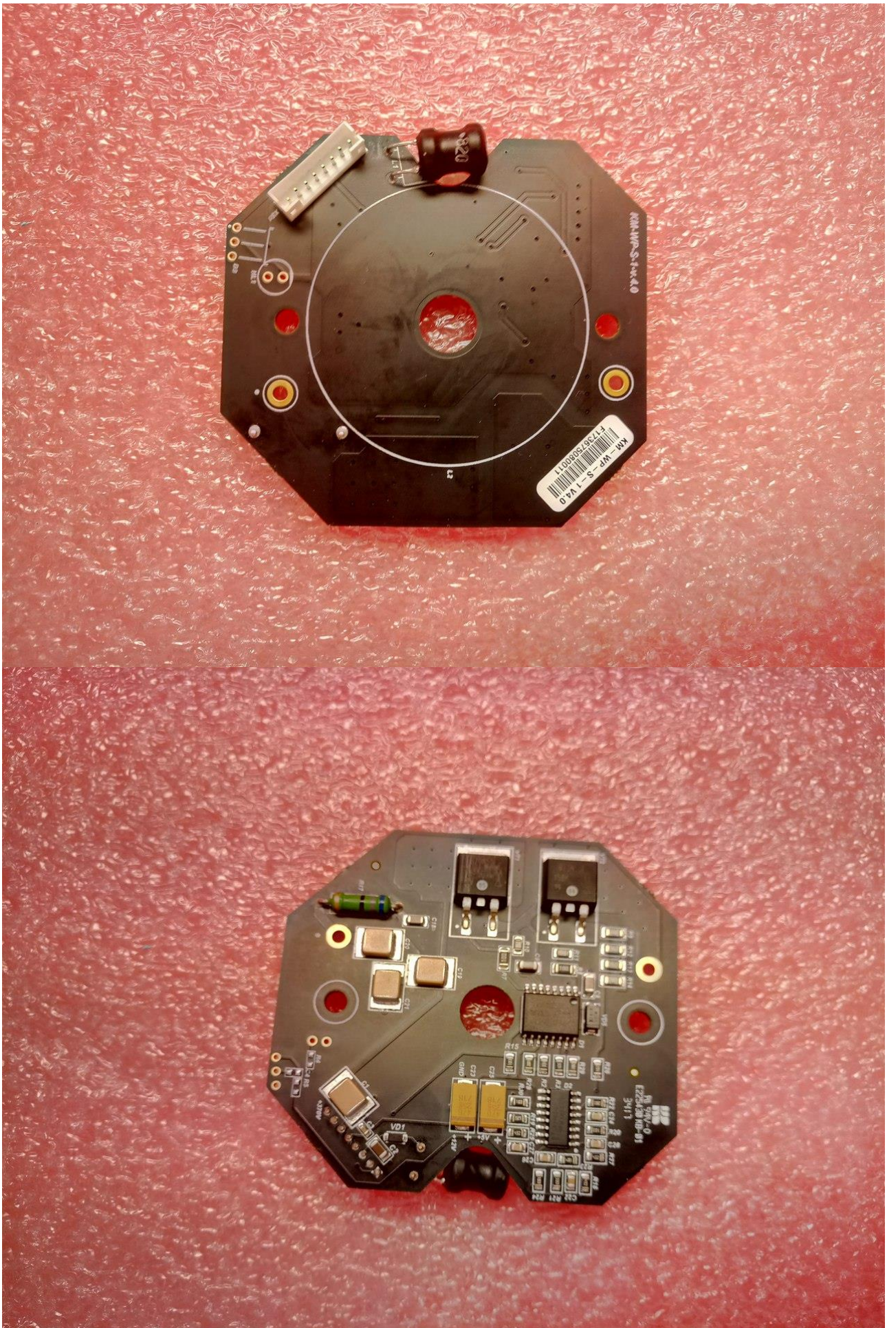
Fig 6. KM-WP-S
