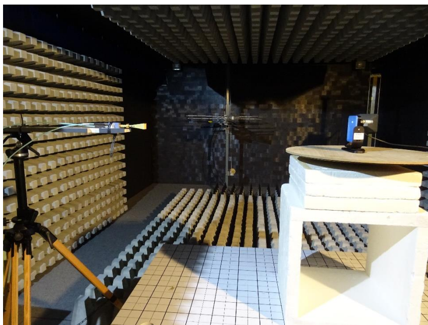
Photo 10 Radiated Test Setup above 40 GHz
