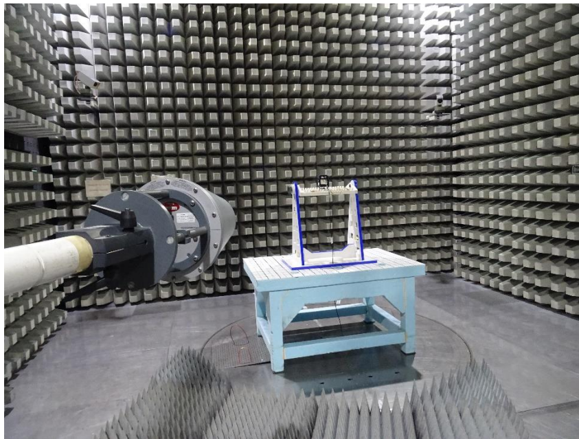
Photo 5 Radiated Test Setup 1 - 18 GHz
