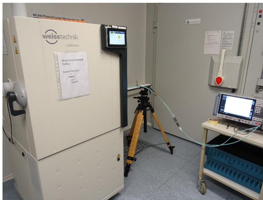
Photo 12 Test Setup frequency stability
