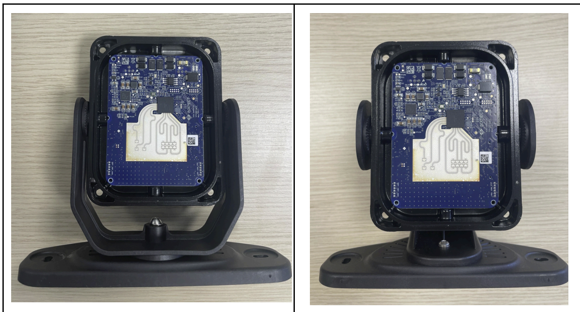
Figure 1: front view without cover with 2-axis rotating stirrup (on the left) and 3-axis rotation stirrup (on the right)
