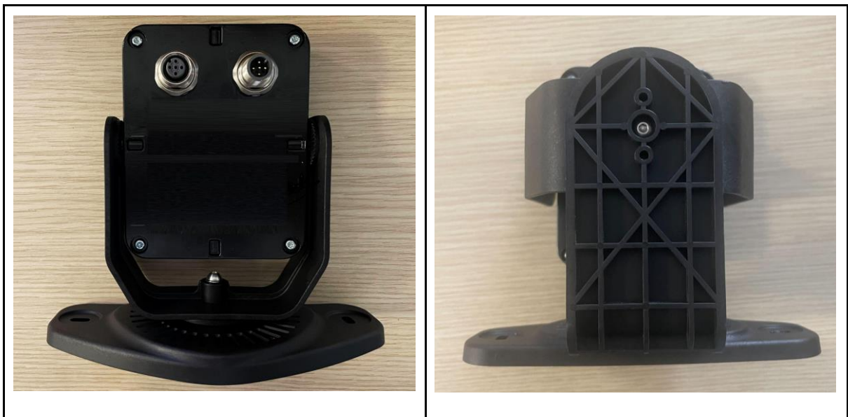
Figure 2: Back view with 2-axis rotating stirrup (on the left) and 3-axis rotation stirrup (on the right)
