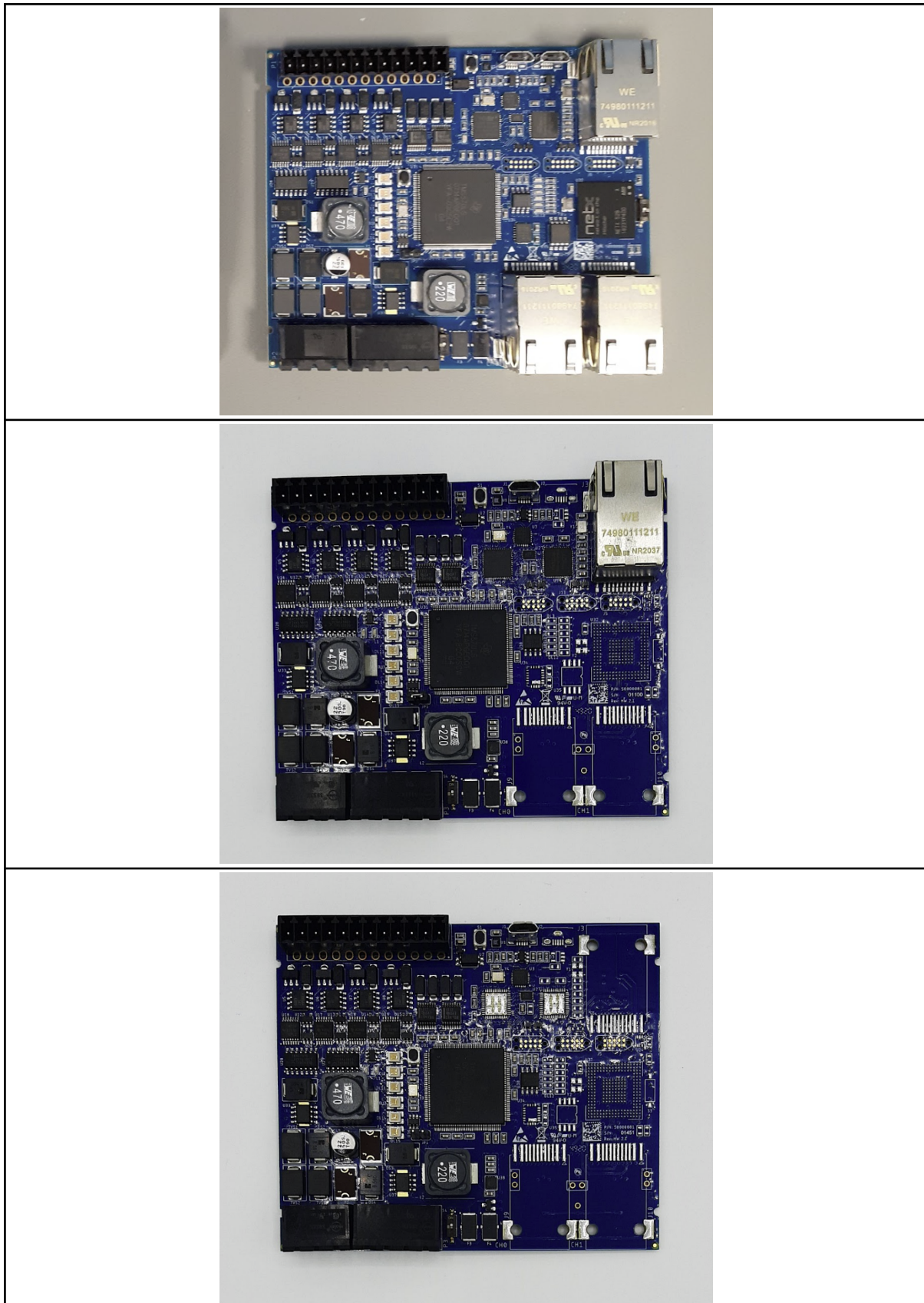
Figure 1: TOP view of ISC-B01 (top image), ISC-02 (middle image) and ISC-03 (bottom image) boards. Images are different because the PCB is the same but ISC-02 and ISC-03 are less populated than ISC-B01.
