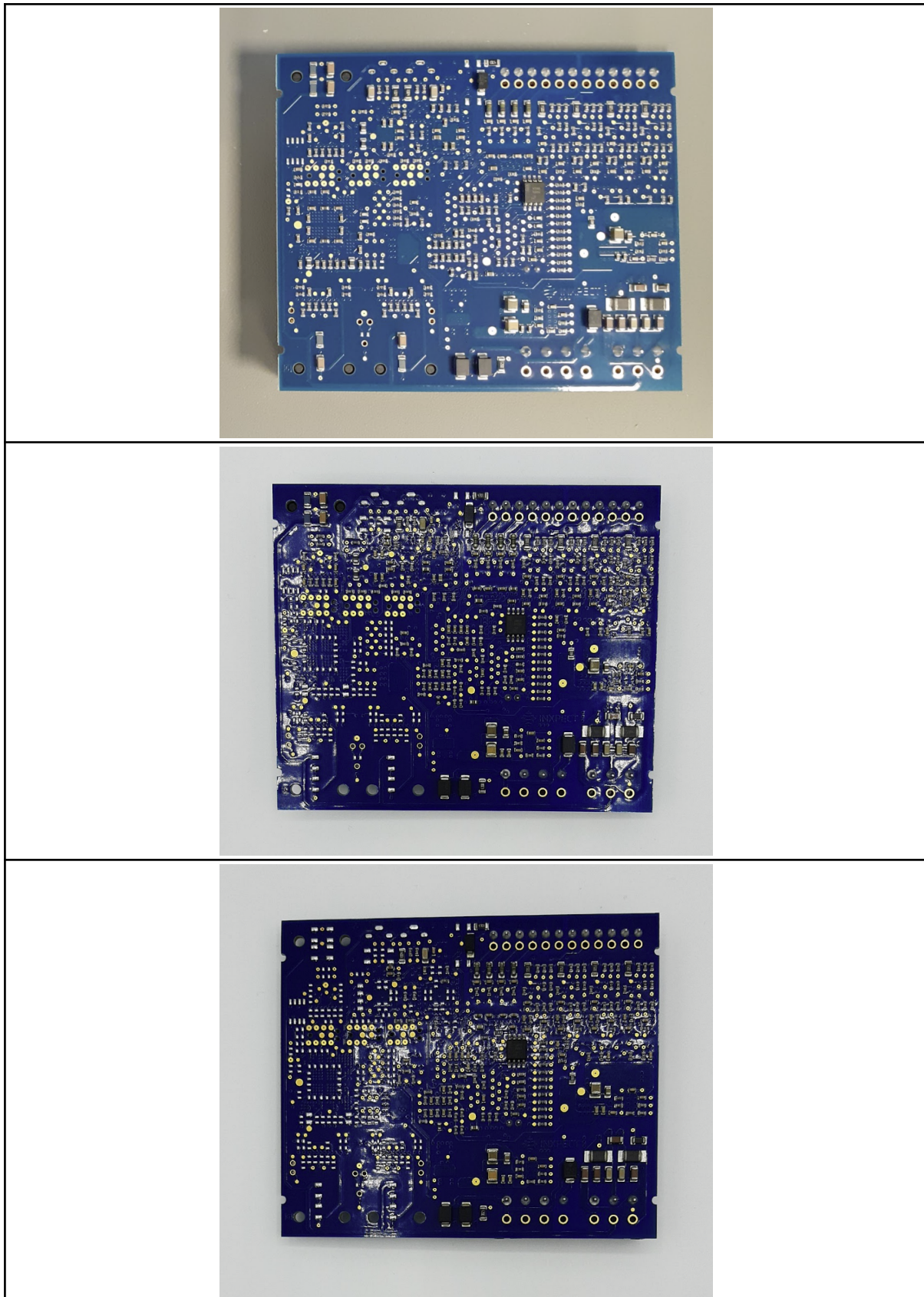
Figure 2: BOTTOM view of ISC-B01 (top image), ISC-02 (middle image) and ISC-03 (bottom image). Images are different because the PCB is the same but ISC-02 and ISC-03 are less populated than ISC-B01.
