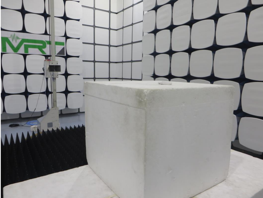
Photograph 3: Set-up for Spurious Emissions of above 1GHz
