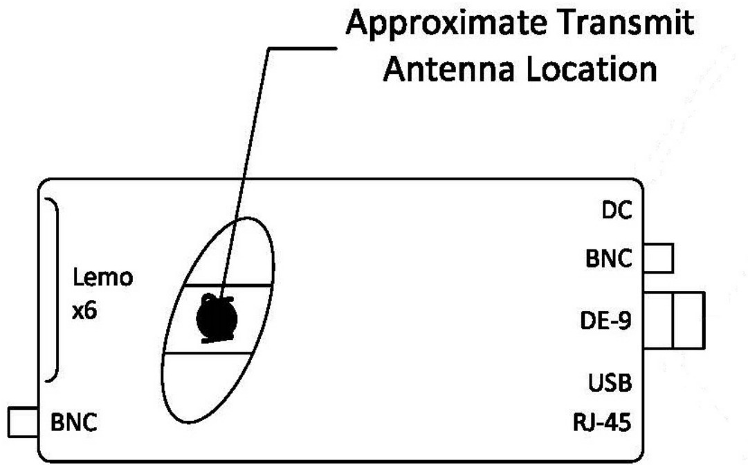
Figure 8.1 SAR Location Diagram of Antenna Distances
