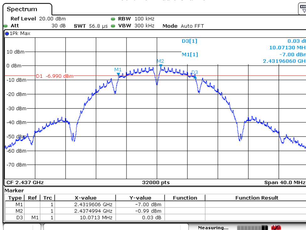
802.11b-Middle Channel
