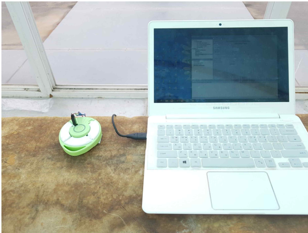
Radiated Emission Test (Below 1 GHz) Close-up of test setup
