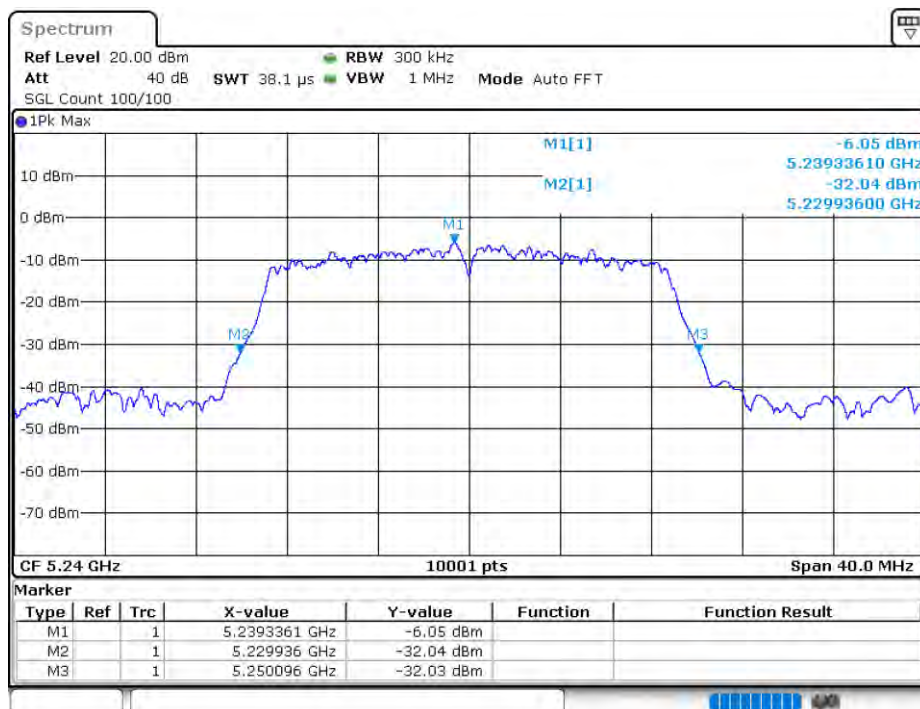
-26 dB BW NVNT 802.11ac20 5240MHz Ant1
