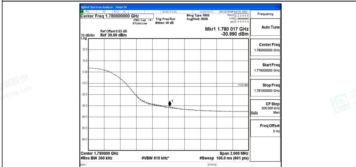
Band66-20MHz-QPSK-132072-100RB#0
