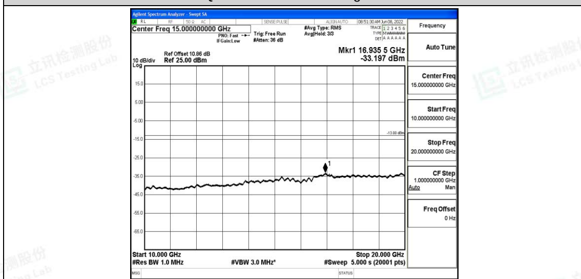
Band4-20MHz-16QAM-20300-1RB#0-Range5:10000~20000MHz
