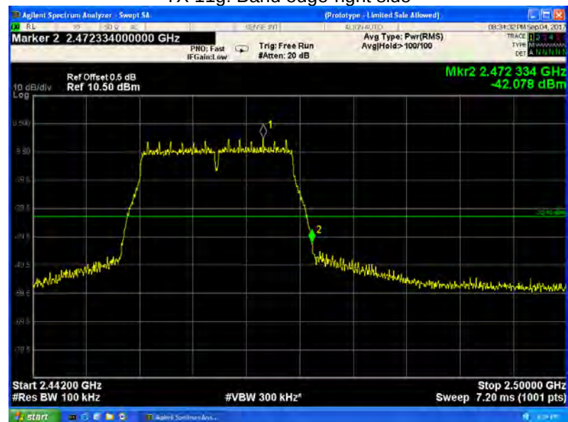
TX 11g: Band edge-right side
