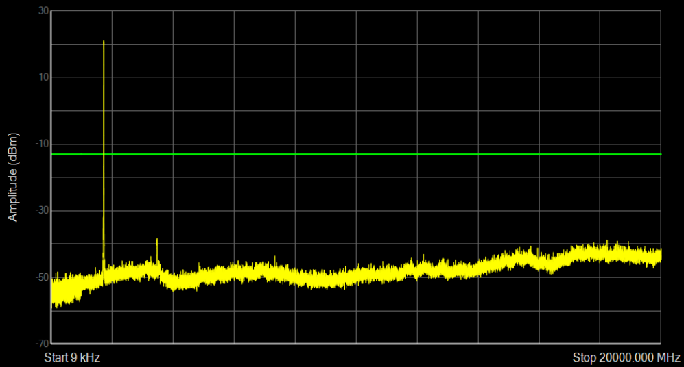
Band66 QPSK BW=5MHz Channel=132322 RB Size=25 Position=#0
